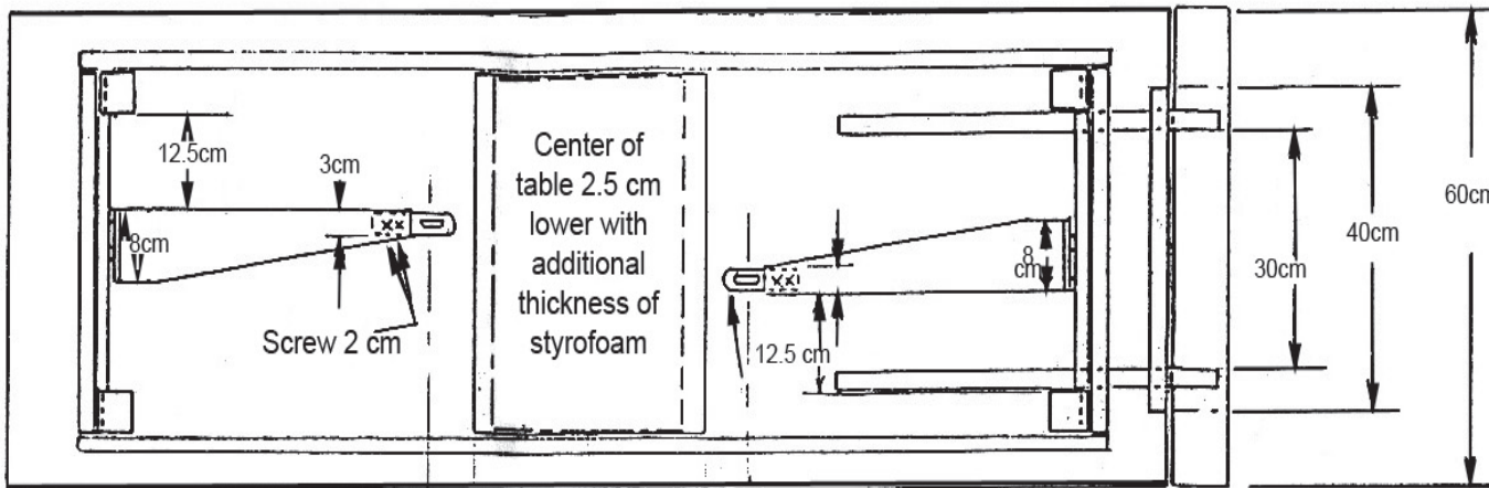
PLAN (UNDERVIEW)
